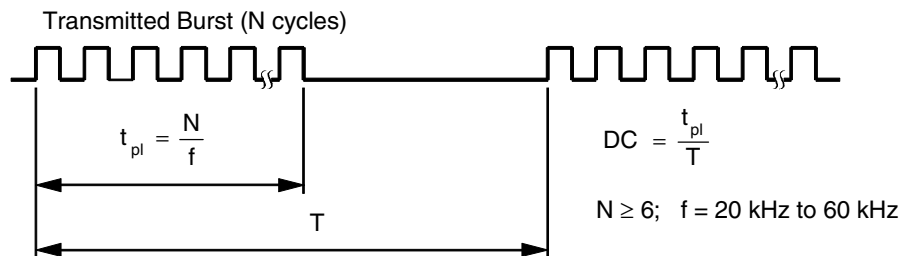
Figure 4. Duty Cycle
