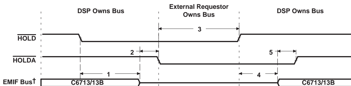
Figure 45. HOLD/HOLDA Timing
