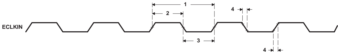
Figure 32. ECLKIN Timings
