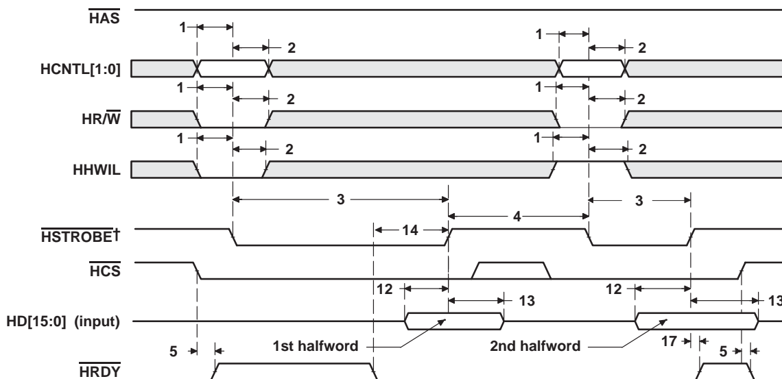
Figure 55. HPI Write Timing ( \overline{\text{HAS}} Not Used, Tied High)
