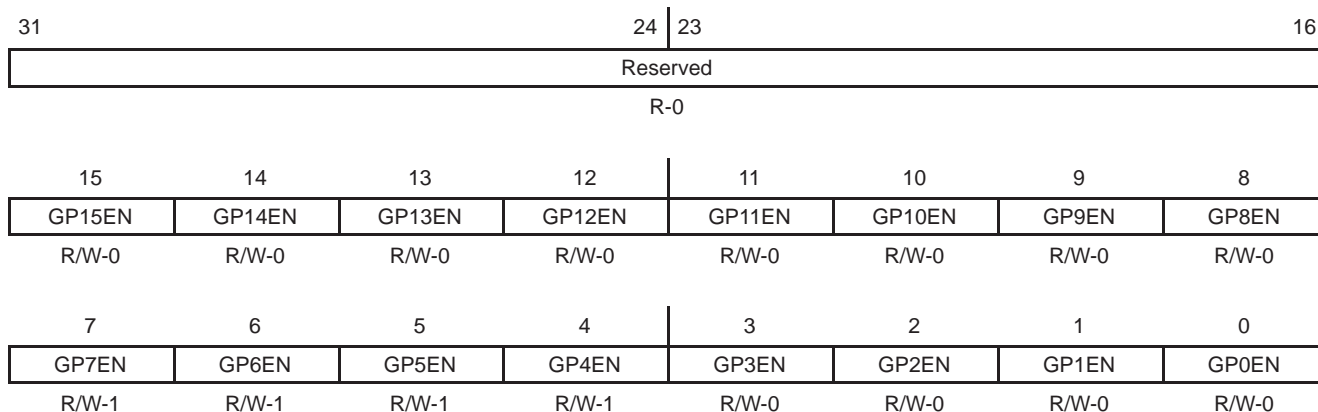
Figure 18. GPIO Enable Register (GPEN) [Hex Address: 01B0 0000]
