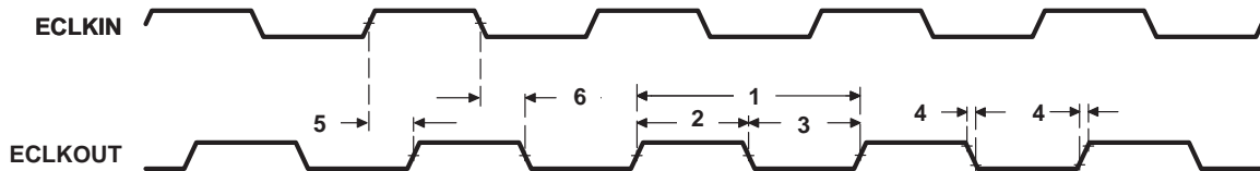
Figure 33. ECLKOUT Timings
