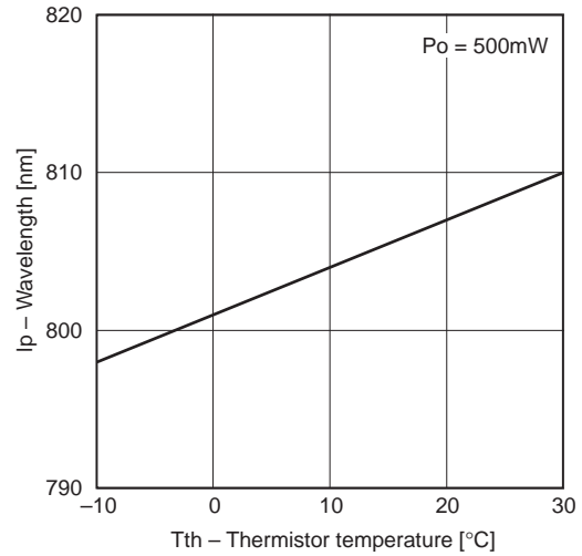
Thermistor characteristics
