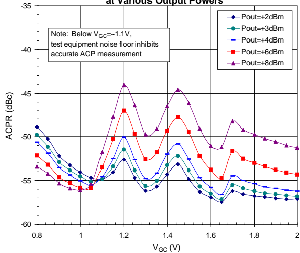
W-CDMA ACPR versus V_{GC} at Various Output Powers
