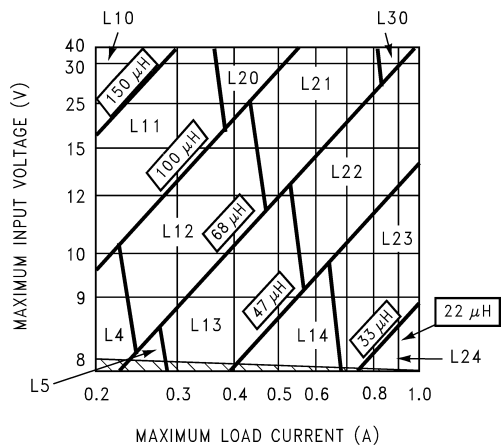
FIGURE 5. LM2675-5.0
