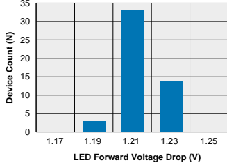
LBA127 Typical LED Forward Voltage Drop (N=50 Ambient Temperature = 25°C; I F = 5mADC)
