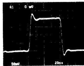
V_{IN} = \pm 10\text{ mV} V_O = \pm 100\text{ mV} 2039-15
