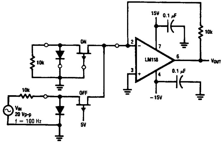
Cross Talk Test Circuit
