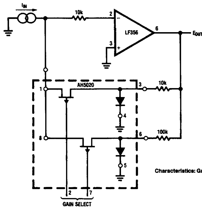
Gain Programmable Amplifier
