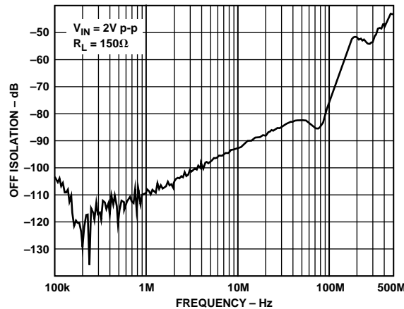
Figure 22. AD8110 Off Isolation, Input-Output
