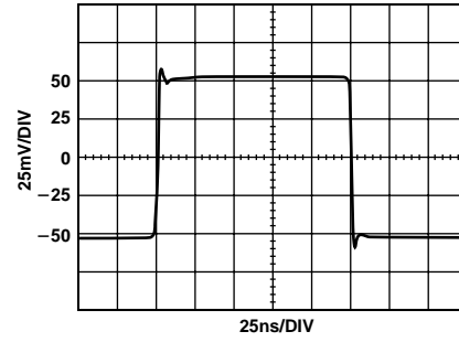
Figure 15. AD8111 Step Response, 100 mV Step
