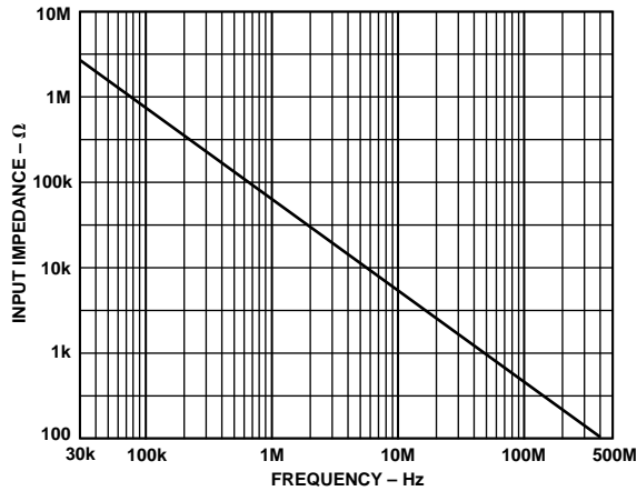
Figure 30. AD8110 Input Impedance vs. Frequency
