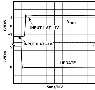
Figure 39. AD8111 Switching Time
