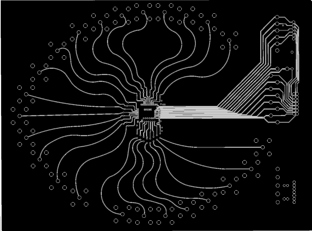
Figure 47. Board Layout (Signal Layer)
