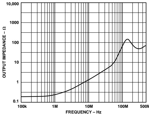
Figure 23. AD8110 Output Impedance, Enabled
