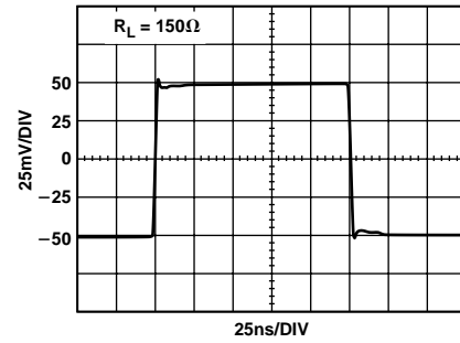
Figure 9. AD8110 Step Response, 100 mV Step
