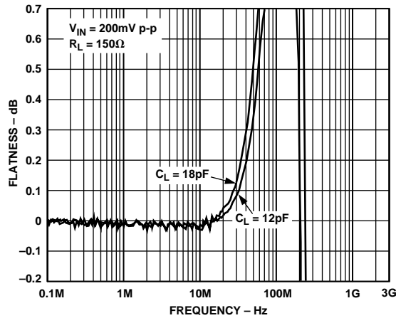
Figure 32. AD8110 Flatness vs. Capacitive Load
