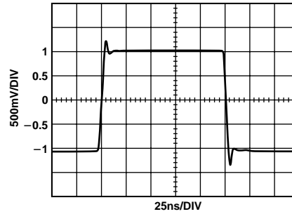
Figure 16. AD8111 Step Response, 2 V Step
