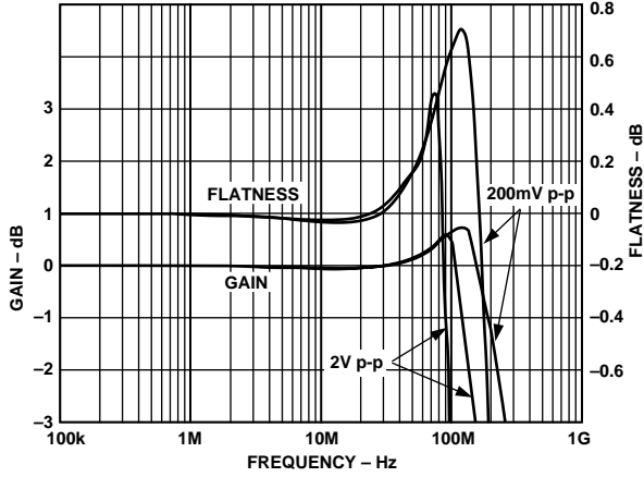
Figure 12. AD8111 Frequency Response
