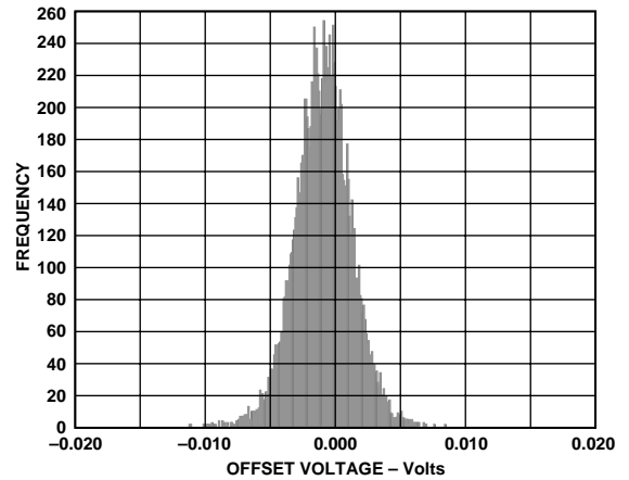
Figure 34. AD8110 Offset Voltage Distribution
