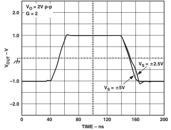
TPC 28. Large Signal Transient Response vs. V_S . See Test Circuit 1.
