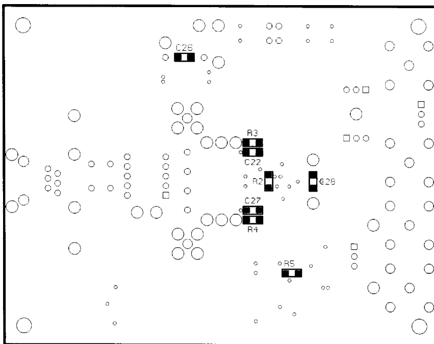
Figure 19. Assembly—Secondary Side
